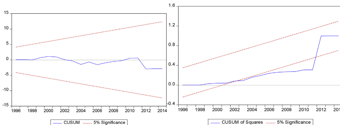
Fig. 5. Stability test for model Energy Consumption.
