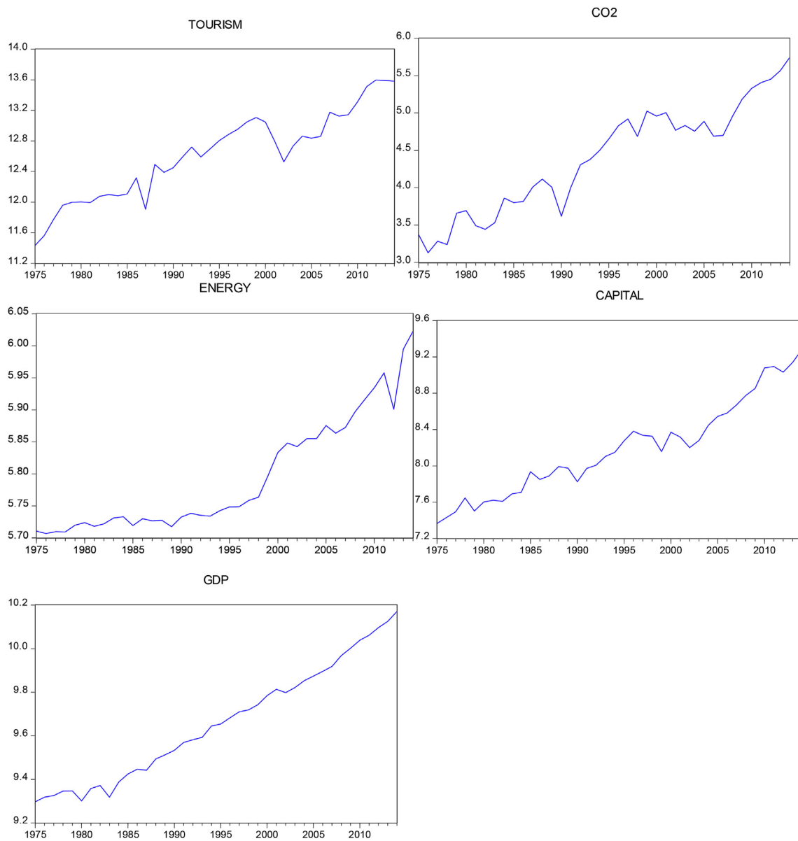
Fig. 1. Trends in the transformed variables.
