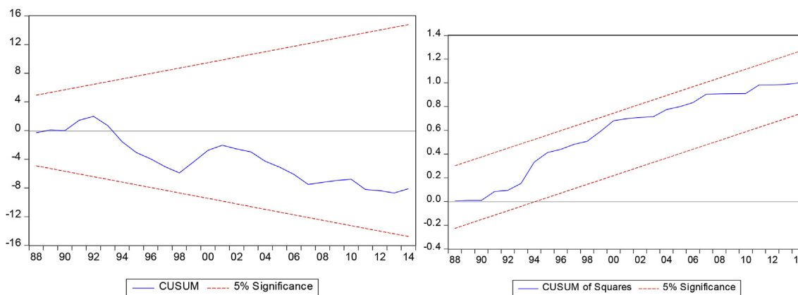
Fig. 4. Stability test for model GDP.
