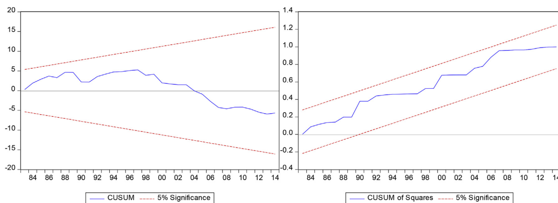
Fig. 2. Stability test for model CO 2 emissions.
