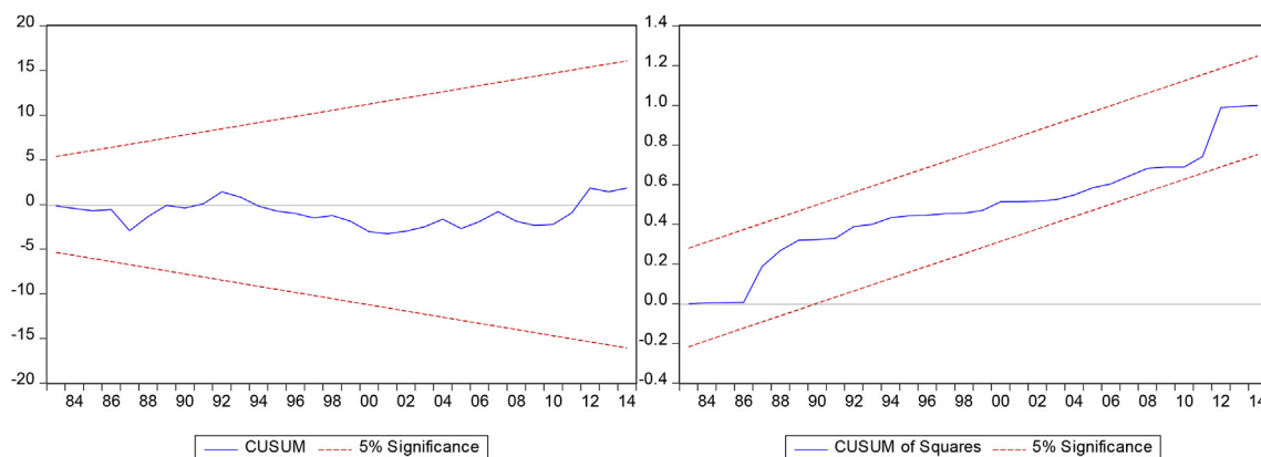
Fig. 3. Stability test for model tourist arrivals.
